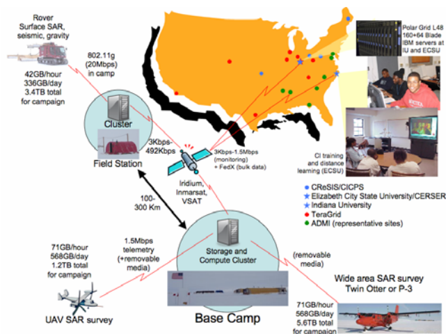
Fig. 1. PolarGrid's major components and concept of operations.
